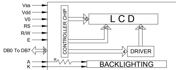
BLOCK DIAGRAM
