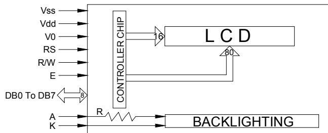
BLOCK DIAGRAM
